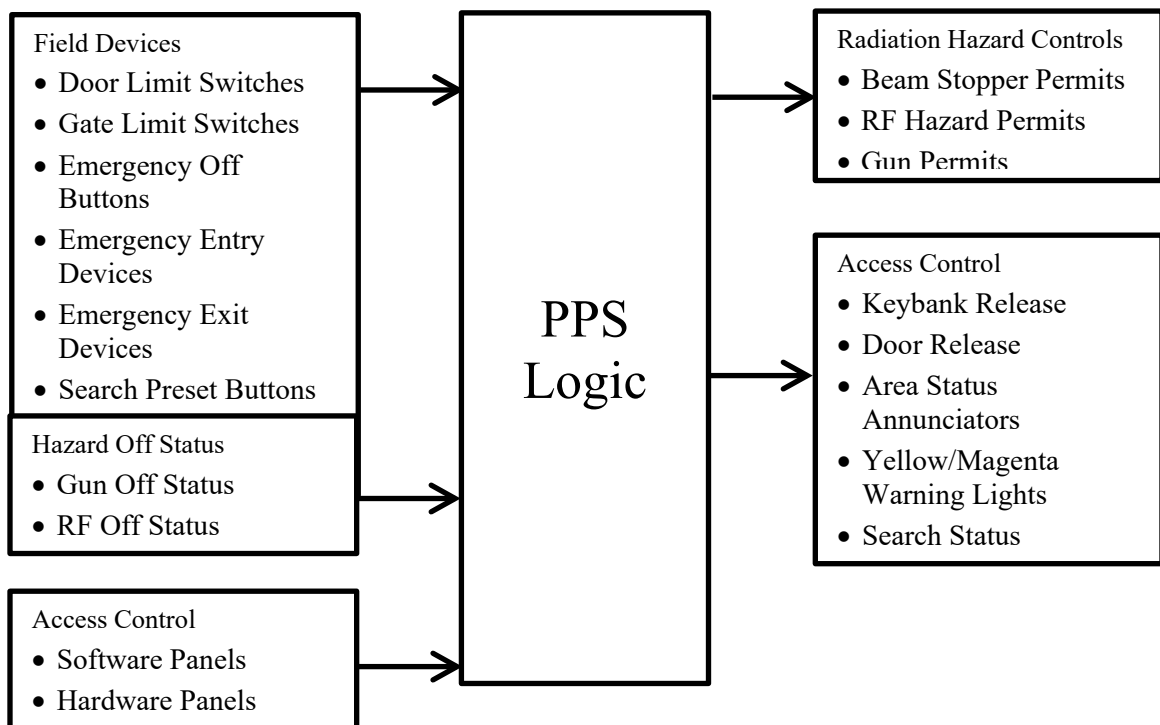
Figure 4-1 PPS System Information Flow
